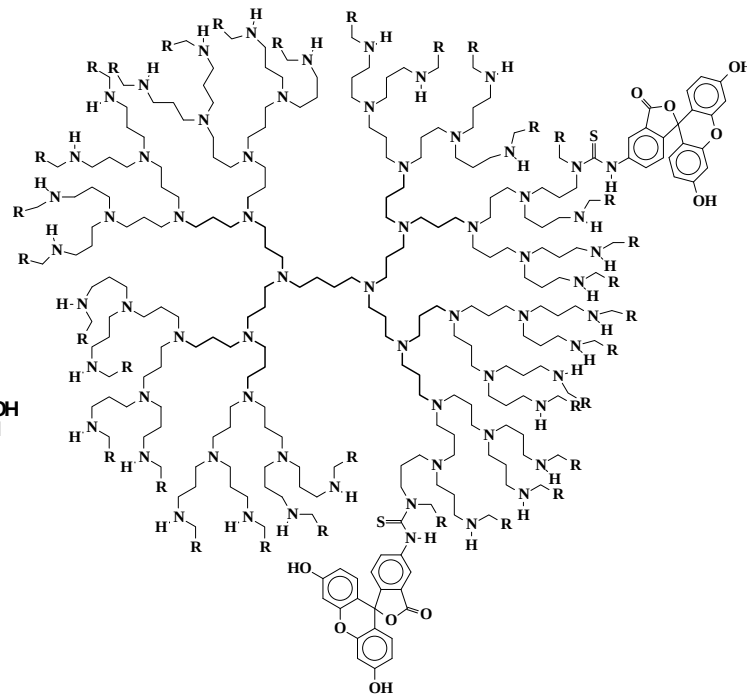
Structure type B Mono-substituted
