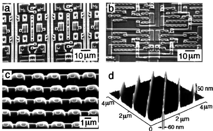
Figure 9 SEM and AFM images of polymeric microstructures fabricated using SAMIM (25). (a–c) SEM images of quasi-three-dimensional structures in photoresist (Microposit 1805, Shipley; \sim 1.6\ \mu\text{m} thick) spin-coated on Si/SiO 2 , polystyrene (PS, Goodfellow; 2.0\ \mu\text{m} thick), and ABS (Goodfellow; 0.85\ \mu\text{m} thick), respectively. (d) An AFM image of nanostructures in a thin ( \sim 0.4\ \text{nm} thick) film of Microposit 1805 spin-coated on Si/SiO 2 . The solvent we used was ethanol for the photoresist and acetone for PS and ABS.
