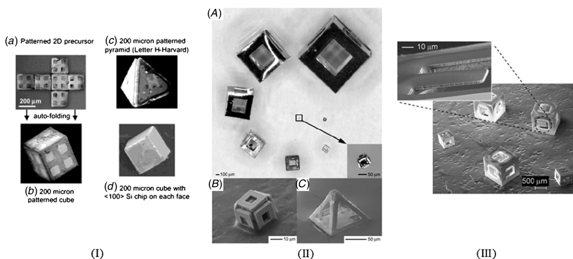
Figure 3. Capillary self-folding of small building blocks. (Ia) Optical microscopy image of a 2D cross; the pattern shown is a contrast between Cr and Au. (Ib) SEM image of a patterned, 200 \mu\text{m} sidelength metallic cube. (Ic) SEM image of a 200 \mu\text{m} sidelength patterned metallic pyramid. (Id) SEM image of a 200 \mu\text{m} sidelength metallic cube containing 340 nm thick \langle 100 \rangle silicon chips on each face. (Reprinted from [29], with permission from Wiley.) (IIA) Optical image showing free-standing polyhedra fabricated with a wide range of sizes all the way from 2 mm to (IIB) 15 \mu\text{m} and with different shapes (e.g. (IIC) square pyramid). (Reprinted from [30], with permission from ACS.) (III) Scanning electron microscope image of self-assembled cubic devices with cantilevers along each of the three axes. A single cantilever is also shown in the zoomed inset. (Reprinted with permission from [31], © 2008 American Institute of Physics.)
