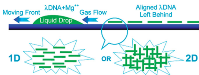
Figure 28. Schematic representation of unidirectional DNA stretching using a droplet. (Reprinted from [190], with permission from ACS.)
