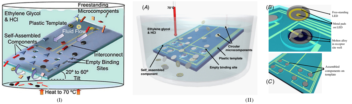
Figure 12. (I) The heterogeneous self-assembly process with shape matching, after Staugh and Parviz. Microcomponents are introduced over a template submerged in a liquid medium and moved with the fluid flow. Self-assembly occurs as microcomponents first fall into complementarily shaped wells and then become bound by the capillary forces resultant from a molten alloy. (Reprinted from [71], © 2006 National Academy of Sciences, USA.) (II) Another view of the process. (B) A microcomponent approaching a binding site with a complementary shape on the template. The molten alloy positioned at the bottom of the binding site on the template wets the metal pads on the microcomponent and forms a mechanical and electrical connection between the microcomponent and the template. (C) Assembled circular microcomponents on a template after the fluidic self-assembly is concluded. (Reprinted from [72], with permission from IOP.)
