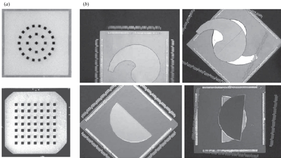
Figure 4. Optical micrographs of capillary-driven self-assembly of flat microparts, after Srinivasan et al. : (a) square parts on quartz substrates in ring and grid configurations and (b) correct and wrong alignments for semicircle- and comma-shaped binding sites. (Reprinted with permission from [6], © 2001 IEEE.)
