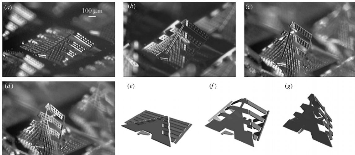
Figure 1. Steps for magnetically driven assembly of out-of-plane microstructures with inside hinge linkage. (a)–(d) Microscope photographs of step-by-step assembly under increasing external magnetic field. (a) Before magnetic field charge. (b) Main part is lifted. (c) Main part is erected. (d) Lock-in part is lifted. (e)–(g) Each step in assembly. (Reprinted with permission from [22], © 2005 IEEE.)
